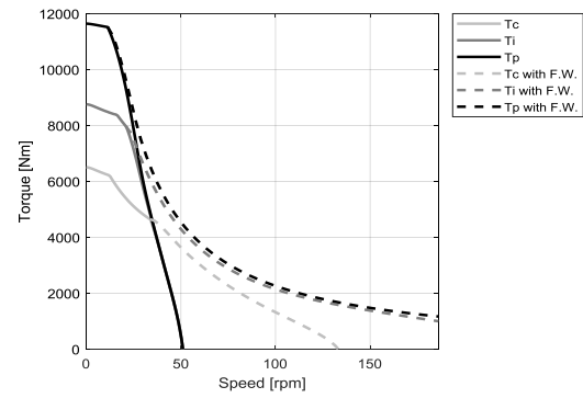
UL - WATER COOLING
