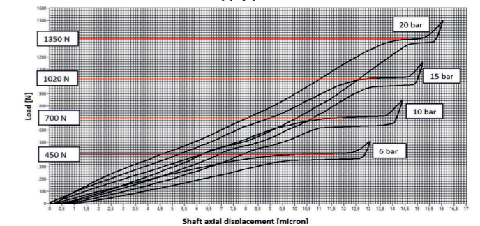
Axial static load capacity at different load supply pressures
