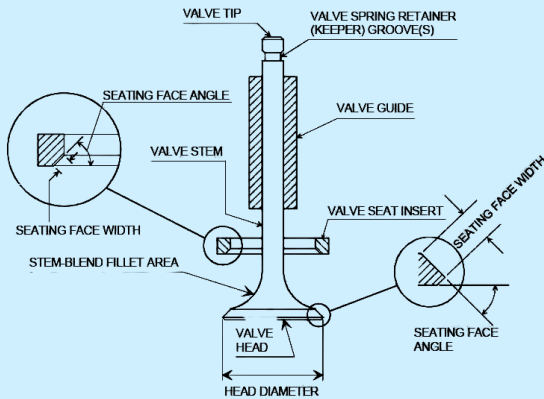
Engine Valve
