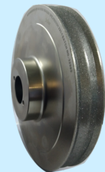
Electroplated Wheel with integral Flange for Kocks Roll Profile Grinding
