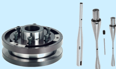
Wheel Flange assembly & Notching spindle for grooving
